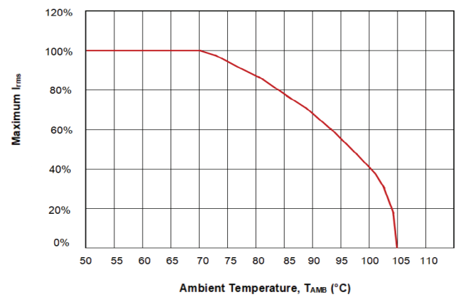
Maximum I_{rms} Vs Ambient Temperature ( T_{AMB} )
